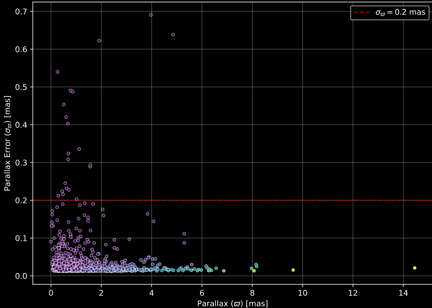
GALAH DR4 Field: [-3] Parallax Quality (n= 1982)
