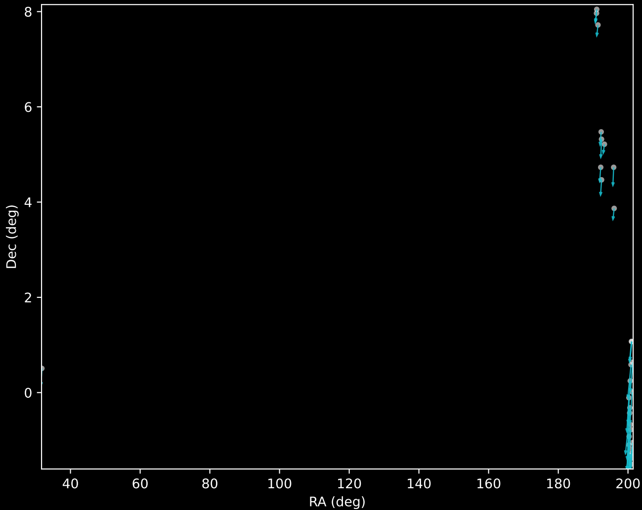
GALAH DR4 Cluster 98 Proper Motion Vectors (n=30)
