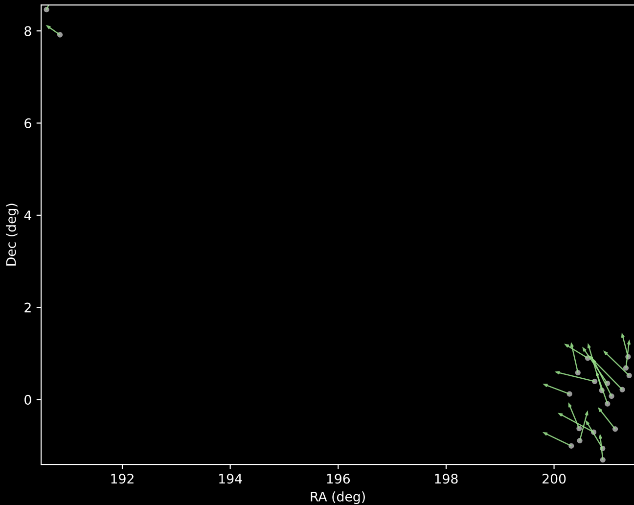
GALAH DR4 Cluster 105 Proper Motion Vectors (n=21)
