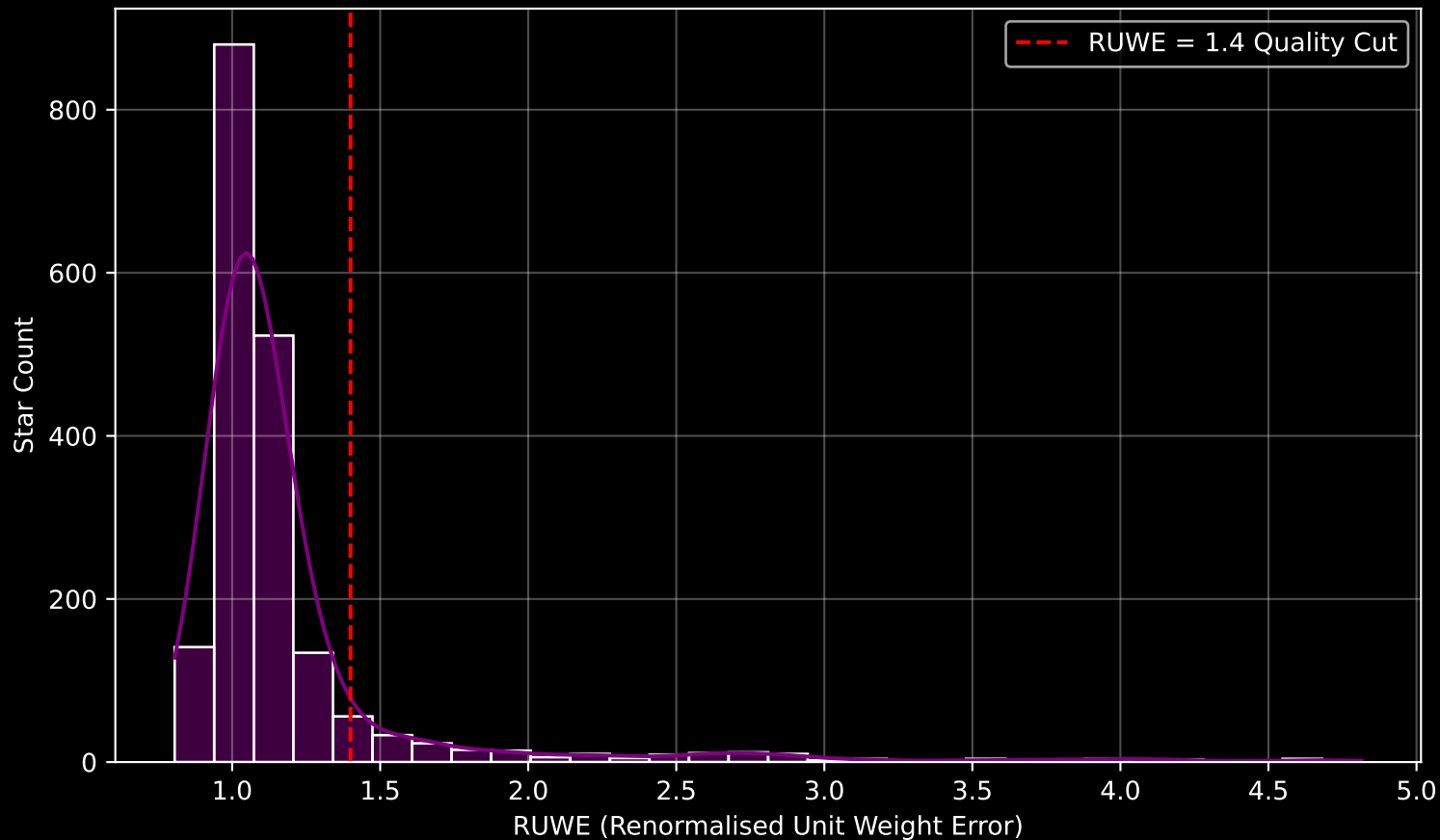
GALAH DR4 Field [-3] RUWE Distribution (n= 1919)
