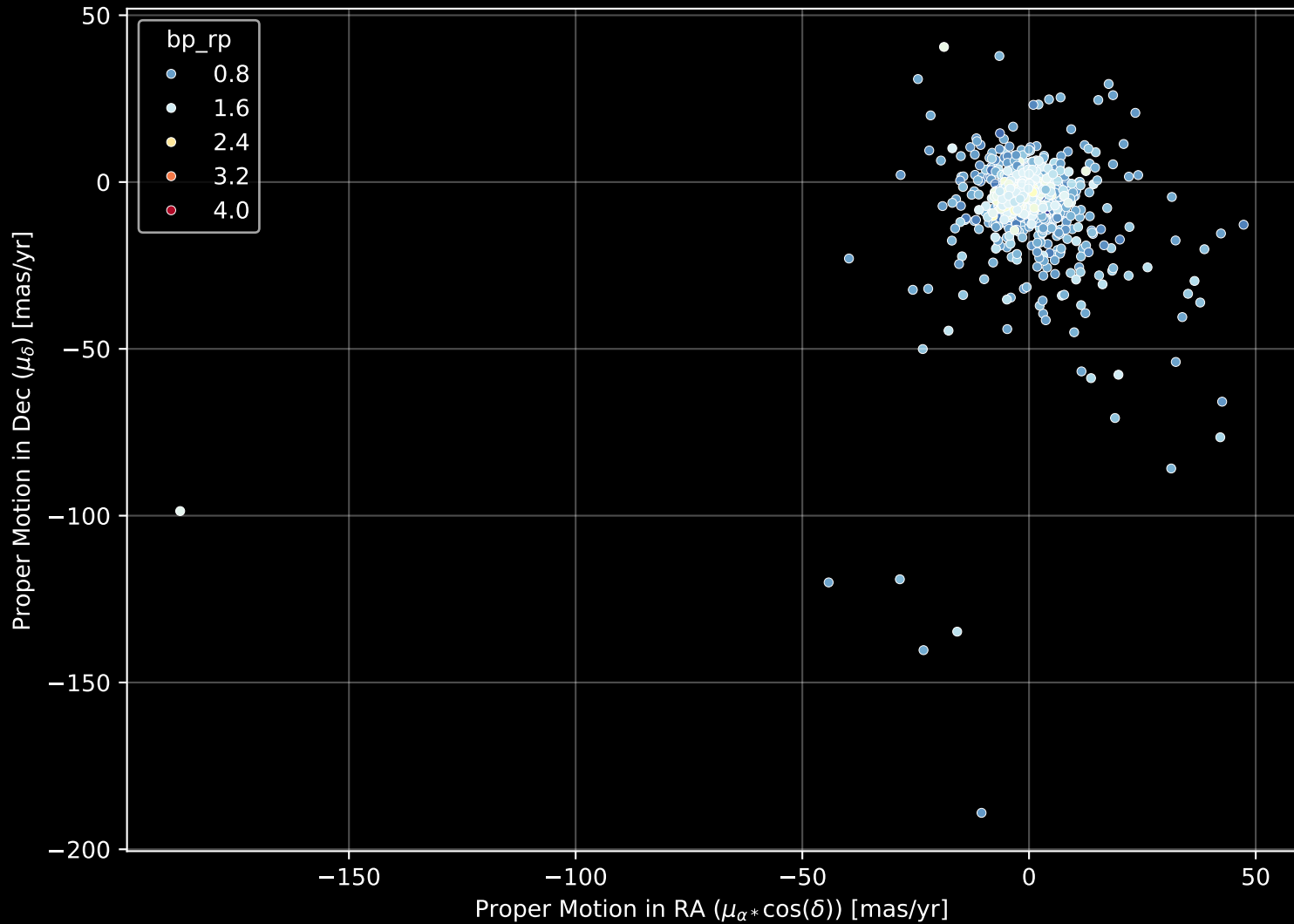
GALAH DR4 Field: [-3] Proper Motion Diagram (n= 1982)
