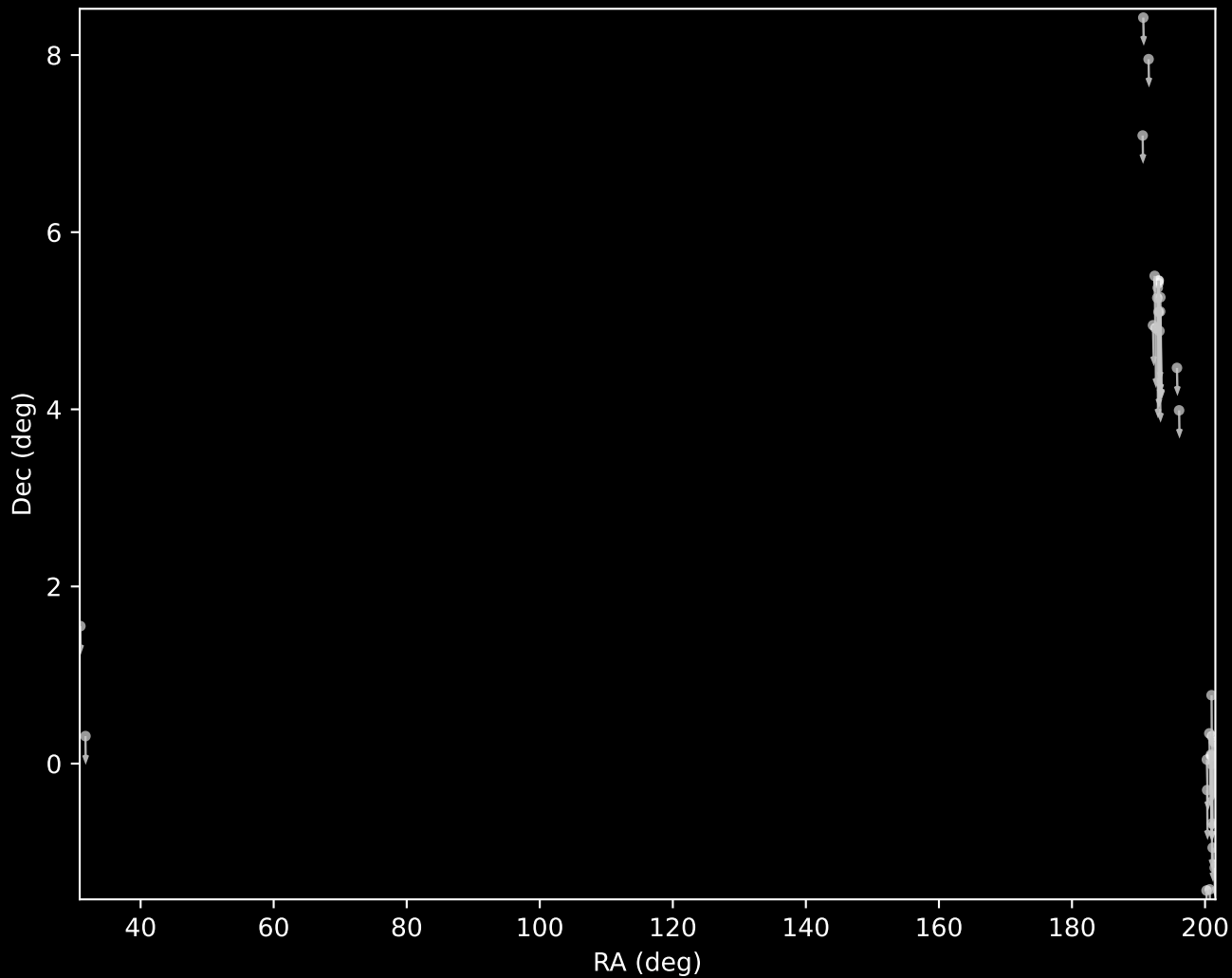
GALAH DR4 Cluster 95 Proper Motion Vectors (n=33)
