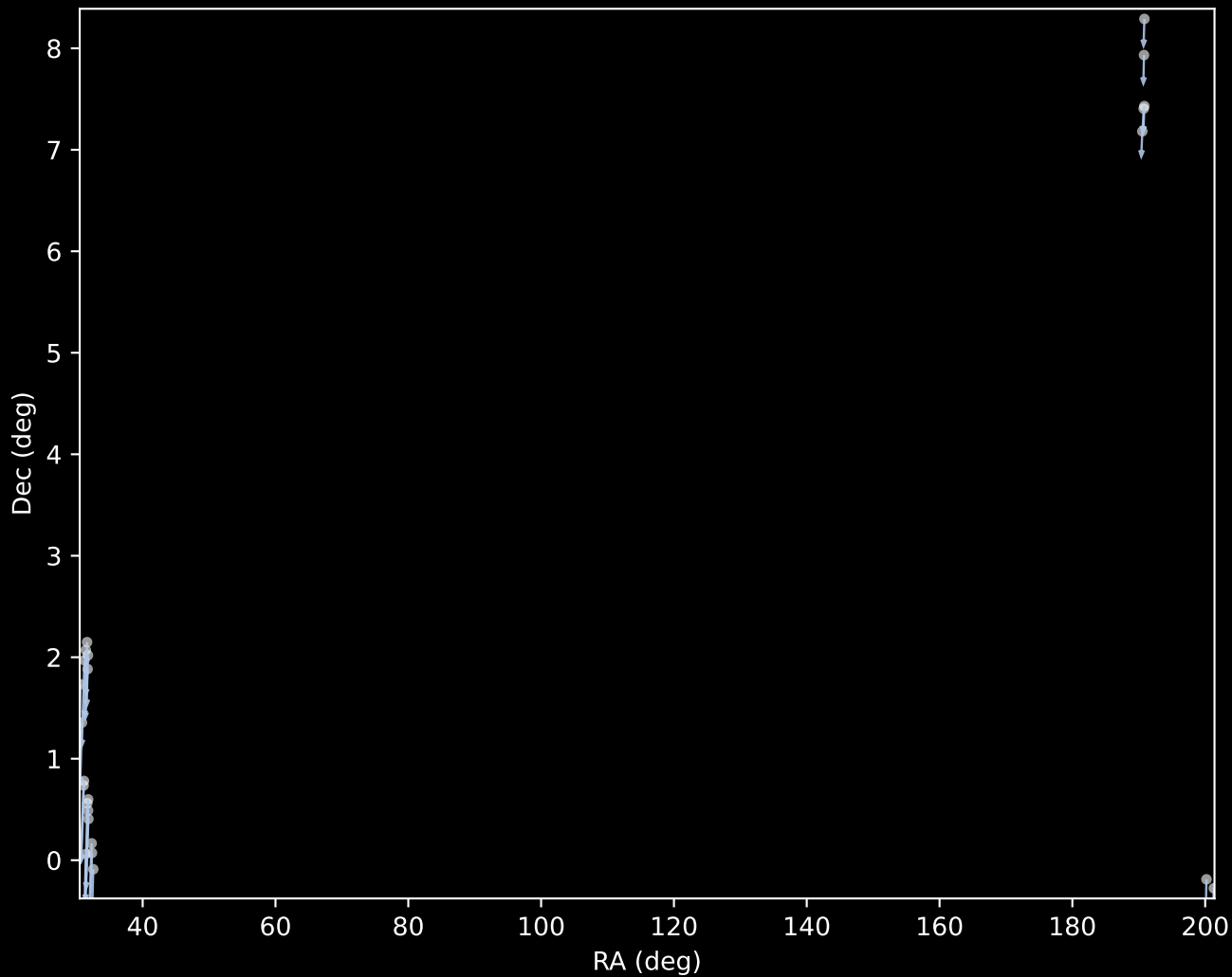
GALAH DR4 Cluster 21 Proper Motion Vectors (n=24)
