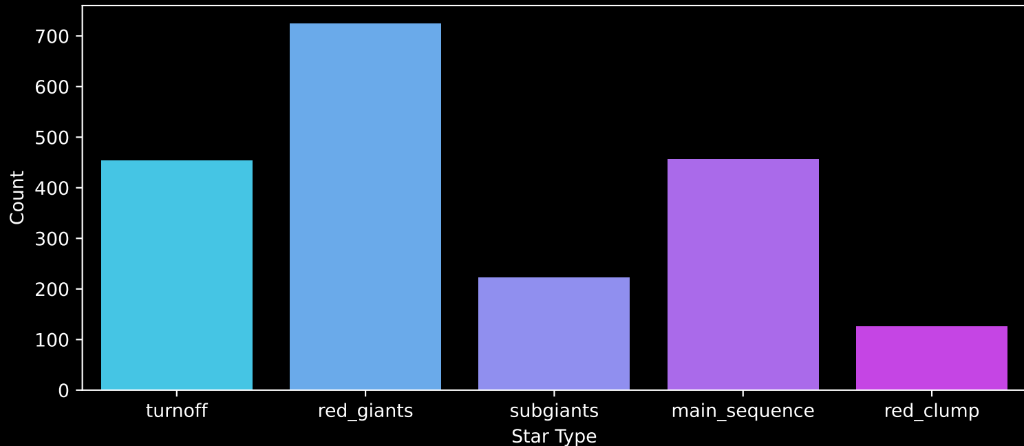
GALAH DR4 Field: [-3] Count plot of Star Type
