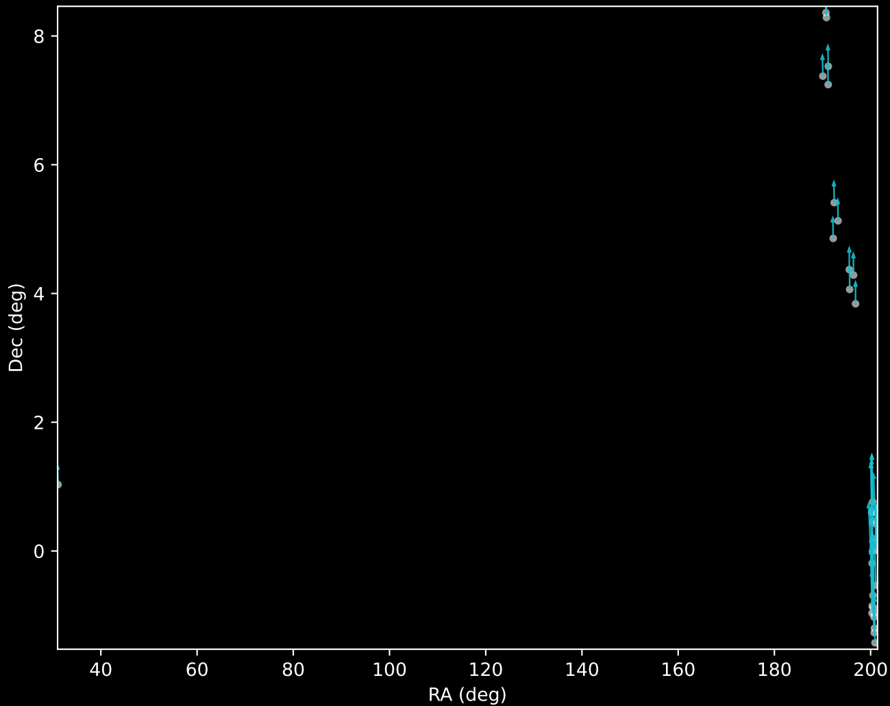
GALAH DR4 Cluster 38 Proper Motion Vectors (n=34)
