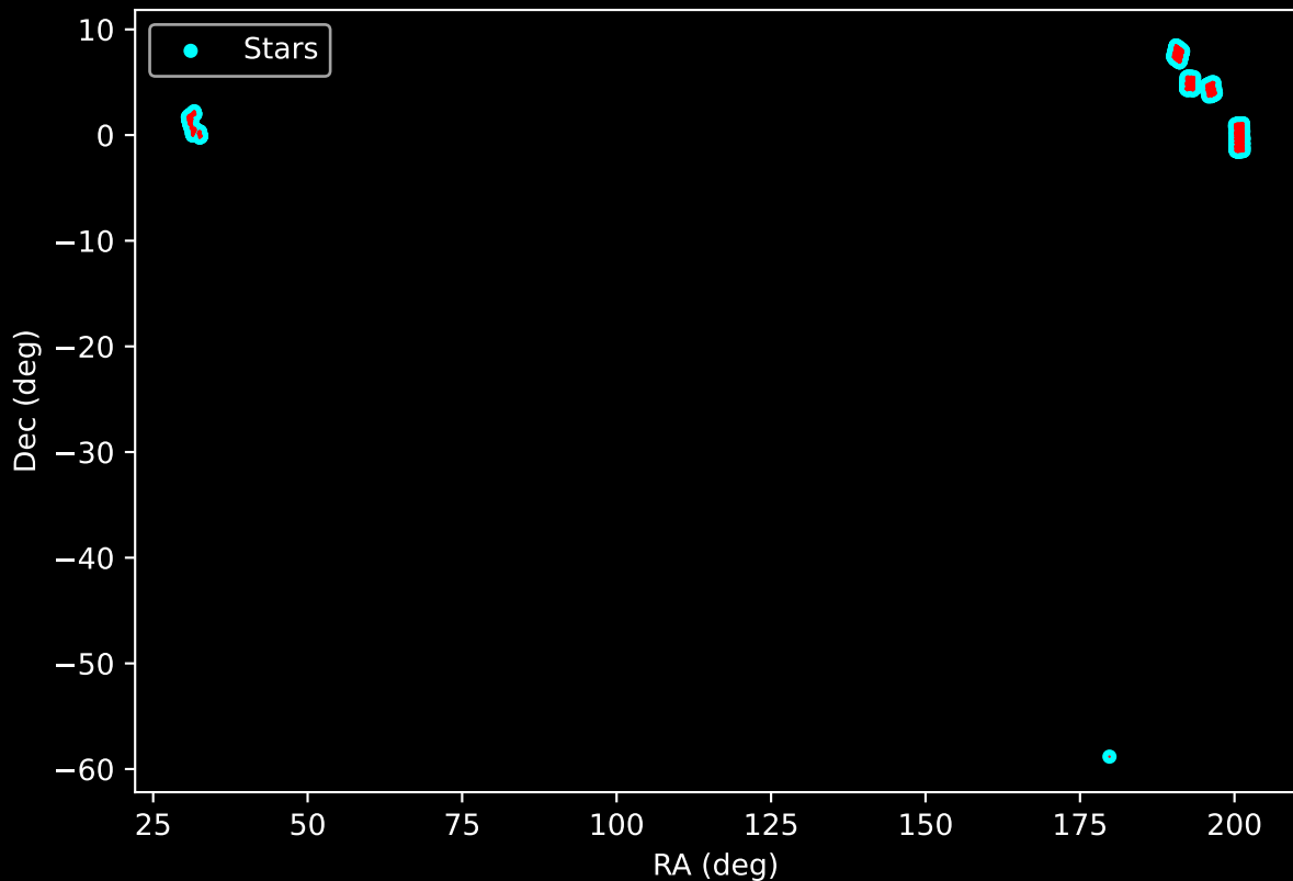
GALAH DR4 Field: [-3] Proper Motion Vectors for Gaia Star Field (n= 1982)
